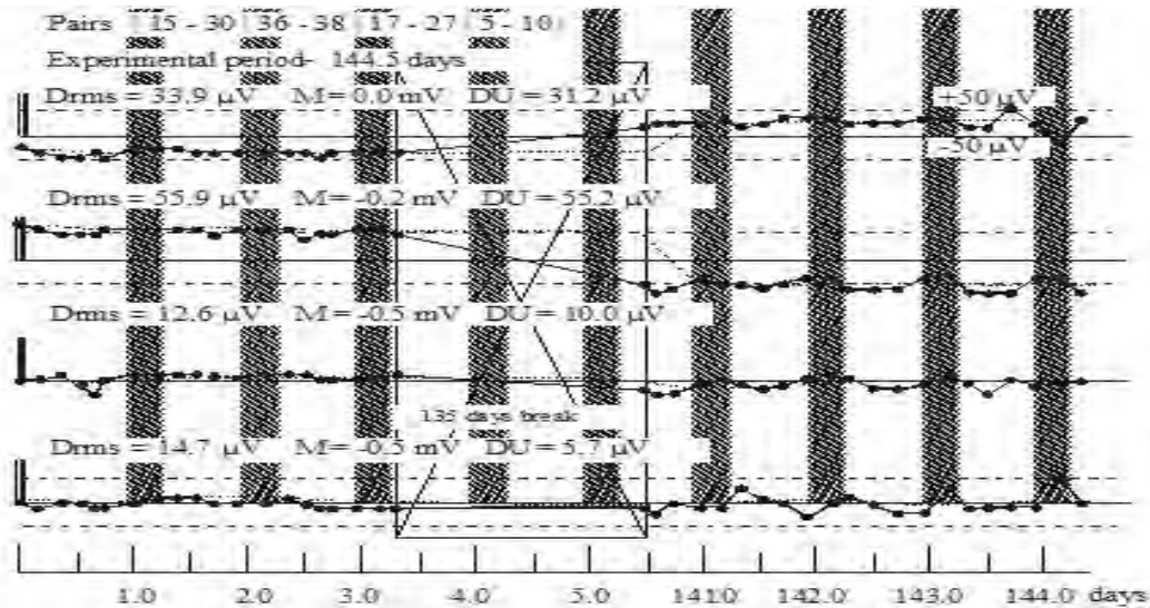
Figure 2: Long-term tests showing approximately 50 \mu V drifting over 144 days.
