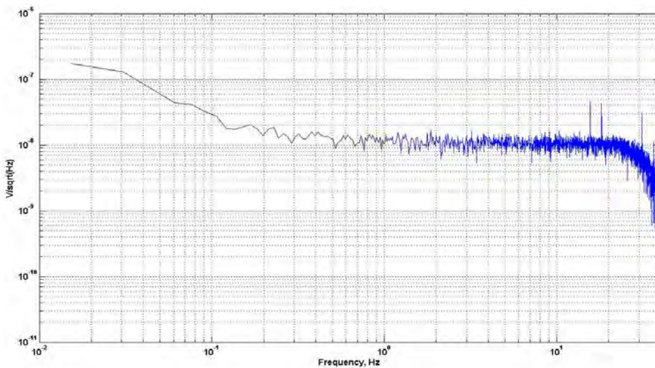
Figure 3: Typical electrode spectral noise density.
