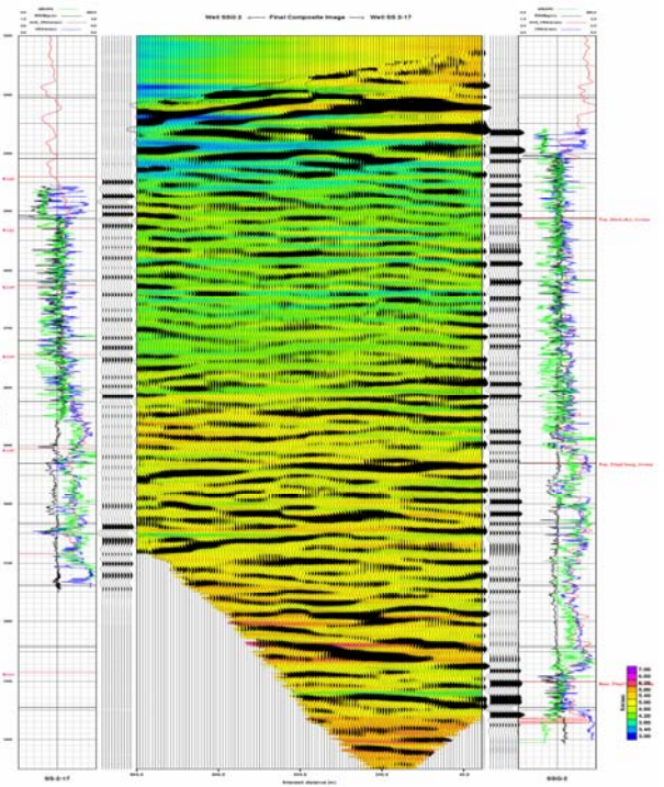
Figure 2: Final composite combined reflection and tomographic inversion image.
