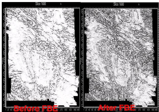
Figure 6 Time slice (1,680 ms) of the Coherence Cube data before FBE (left) and after FBE (right) processing.
