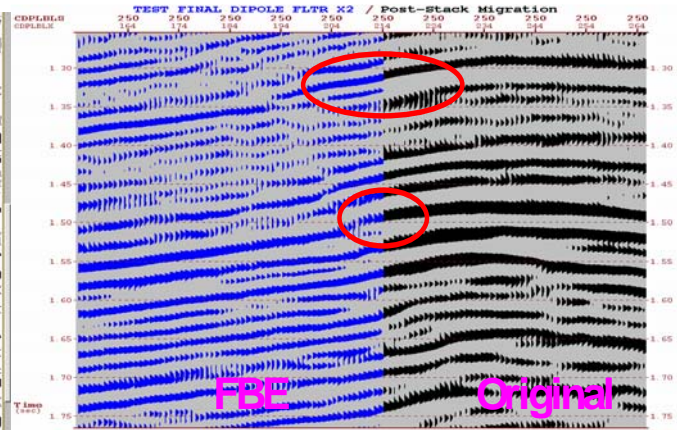
Figure 2 Direct merge of seismic section before FBE (right) and after FBE (left) processing. Additional small reflectors can be identified in red circle areas on FBE data.
