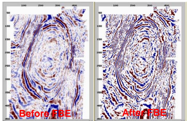
Figure 4 Time slide (1,000 ms) of seismic data before FBE (left) and after FBE (right) processing.
