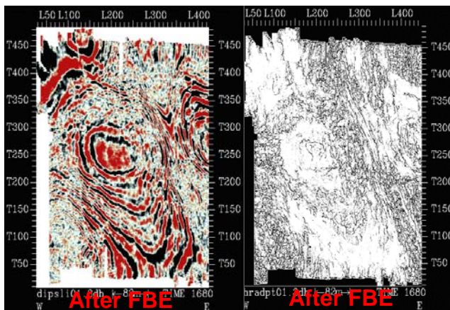
Figure 5 Time slide (1,680 ms) of seismic data (left) and time slide (1,680 ms) of Coherence Cube data (right) comparison.
