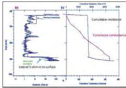
Fig. 6: Example of deriving vertical and horizontal resistivity from an induction log shown on the left. The equivalent values superimposed on the log are derived from the cumulative conductance and cumulative transverse resistance on the right by fitting lines between layer boundaries. The user interactively picks the layer boundaries. The plot was generated with IX1D by Interpex Ltd. ( www.interpex.com ).
