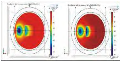
Fig. 10: Electric field response of z-component, E_z observed at the wellbore for Upper Bakken (left) and Lower Bakken (right) at time t = 0.268001 s.
