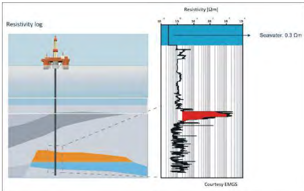
Fig. 2: Sketch of a reservoir in a marine environment and an induction log. The induction log shows high resistivity in the reservoir zone indication high hydrocarbon saturations (courtesy EMGS).
