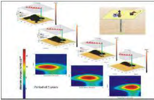
Fig. 18: Simulated response of surface-to-borehole EM for 4 time steps over a period of 5 years (Colombo et al., 2010). For 3 of them the surface-to-borehole anomalous response is shown.
