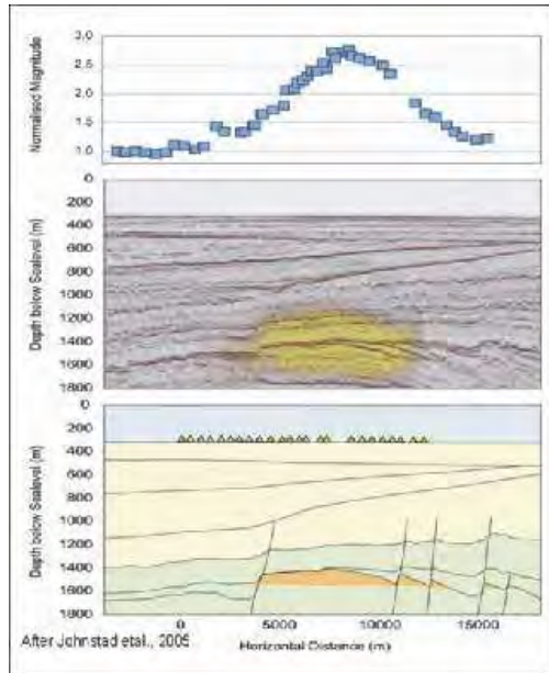
Fig. 7: Example of a marine CSEM interpretation for the Troll field, Norway (after Johnstad et al., 2005). The top shows a magnitude versus offset curve, which exhibits an anomaly directly over the reservoir.
