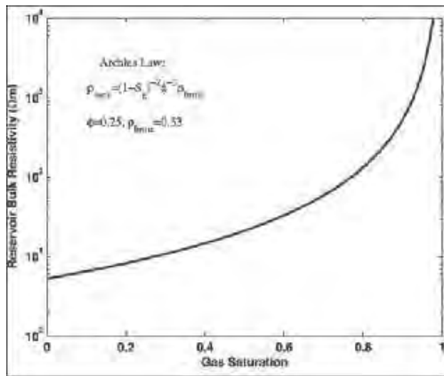
Fig. 1: Reservoir bulk resistivity as a function of gas saturation (Rubin et al., 2006).
