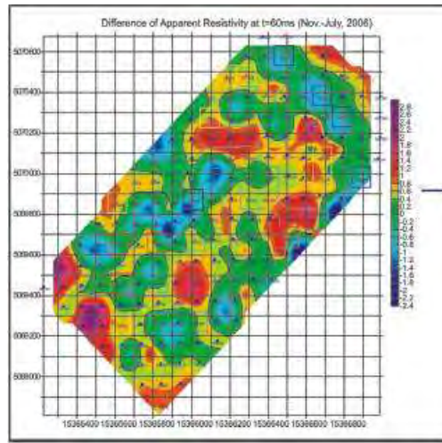
Fig. 17: Time lapse difference map in terms of apparent resistivities from the steam flood driven reservoir monitoring example from China. (Hu et al., 2008).
