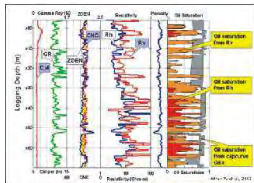
Fig. 5: Example of an interpretation of a 3D induction logs interpretation (Yu et al., 2001). The tracks from left to right show: natural gamma ray for shale content, gamma-gamma density and neutron density for gas zone indicators, 2D inverted vertical and horizontal resistivities, interpreted porosity and interpreted oil saturation.
