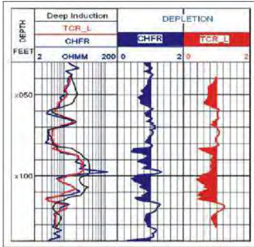
Fig. 16: Steam flood has reduced 80 \Omega -m reservoir resistivity to 40 \Omega -m, black curve represents reservoir resistivity before flooding and red and blue curves represent the resistivity after the reservoir has been flooded (Zhou et al., 2002).
