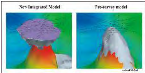
Fig. 11: Interpreted images of the sub-salt exploration survey in Northern Germany. The interpretation integrates magnetotellurics with gravity and seismics (Buehneemann et al., 2002). On the left is the interpretation AFTER acquiring and integrating the MT data and on the right the interpretation before the survey.
