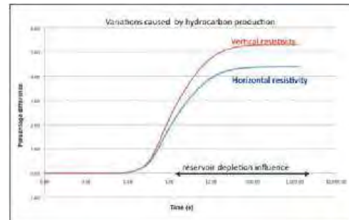
Fig. 19: Time lapse simulation result of 10 % depletion of this horizontal well. The anomaly is still in the 5% range, which is big for long recording times.
